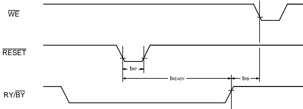
Figure 12 \overline{RESET} , RY/\overline{BY} Timing Diagram
